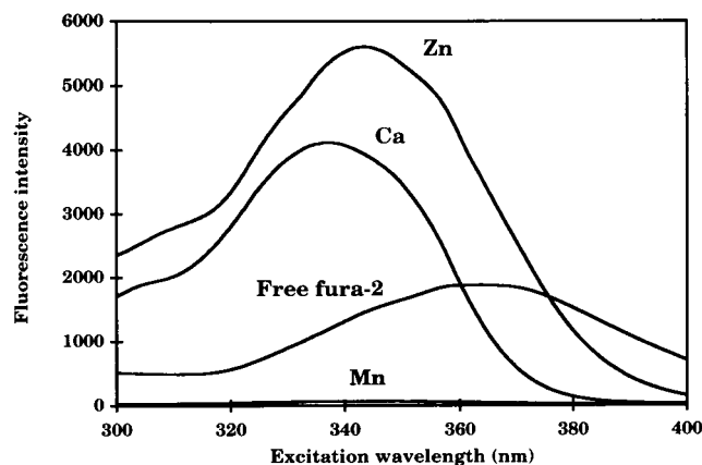
FIGURE 7 Effects of \text{Zn}^{2+} , \text{Ca}^{2+} , \text{Fe}^{2+} , and \text{Mn}^{2+} on the fluorescence excitation spectra of fura-2. Fluorescence excitation spectra of fura-2 (1 \mu M) in \text{Mg}^{2+} -free cytosol-like medium were recorded ( \lambda_{\text{em}} = 510 nm) after addition of 1 mM EGTA (= Free fura-2), \text{CaCl}_2 , \text{MnCl}_2 , \text{ZnCl}_2 , or \text{FeCl}_2 . In the presence of the latter, there was no detectable fluorescence from fura-2.
